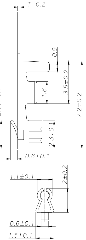
SECTION C-C
