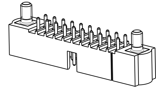
ASSEMBLY M80-50920XX SHOWN FOR ILLUSTRATION PURPOSES ONLY
