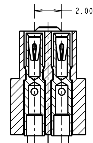
SECTION X-X
