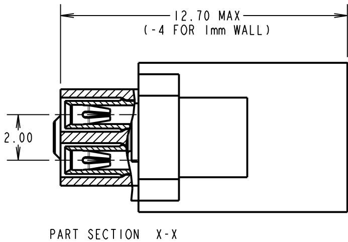
PART SECTION X-X
