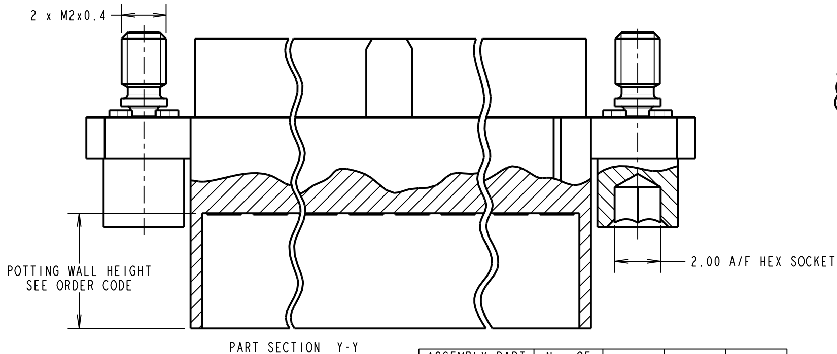
PART SECTION Y-Y
