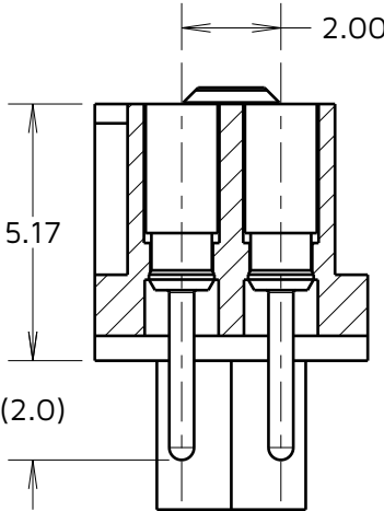
SECTION X-X
