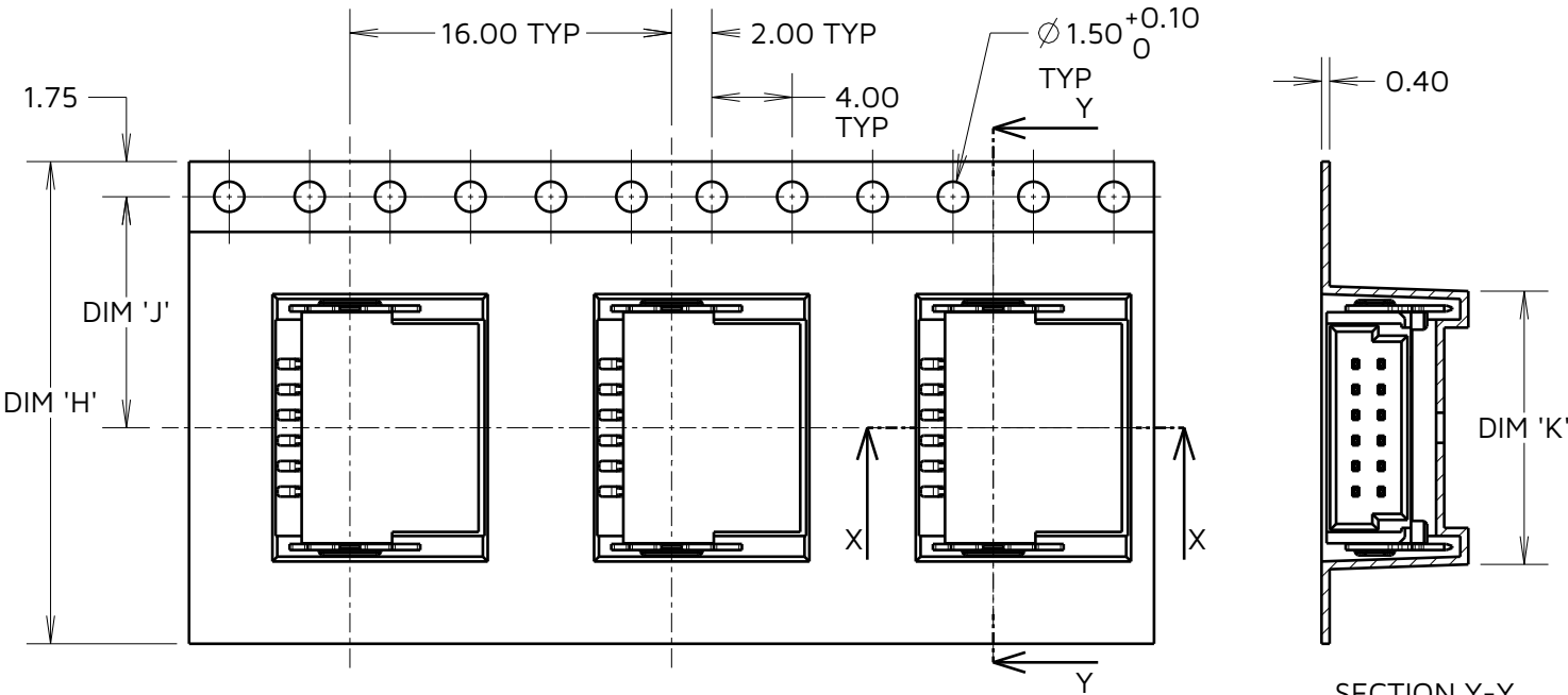
TAPE DETAILS FOR 12 TO 16 CONTACT CONNECTORS
