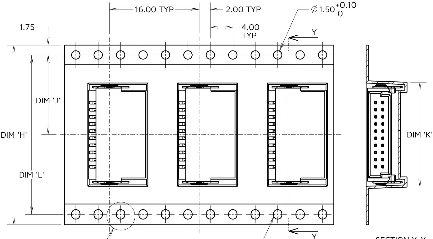
TAPE DETAILS FOR 20 TO 80 CONTACT CONNECTORS
