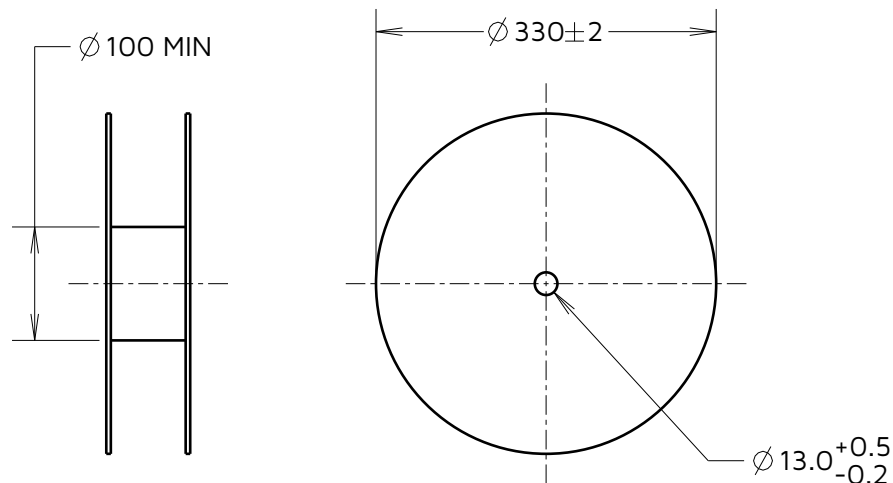
REEL DETAILS
