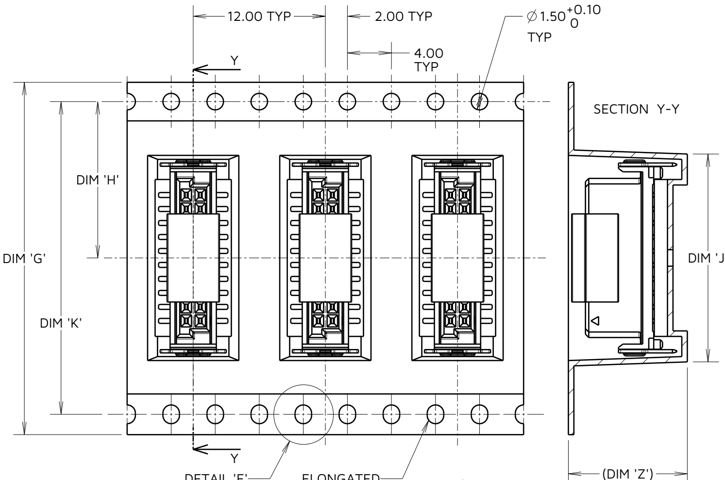
TAPE DETAILS FOR 20 TO 80 CONTACT CONNECTORS
