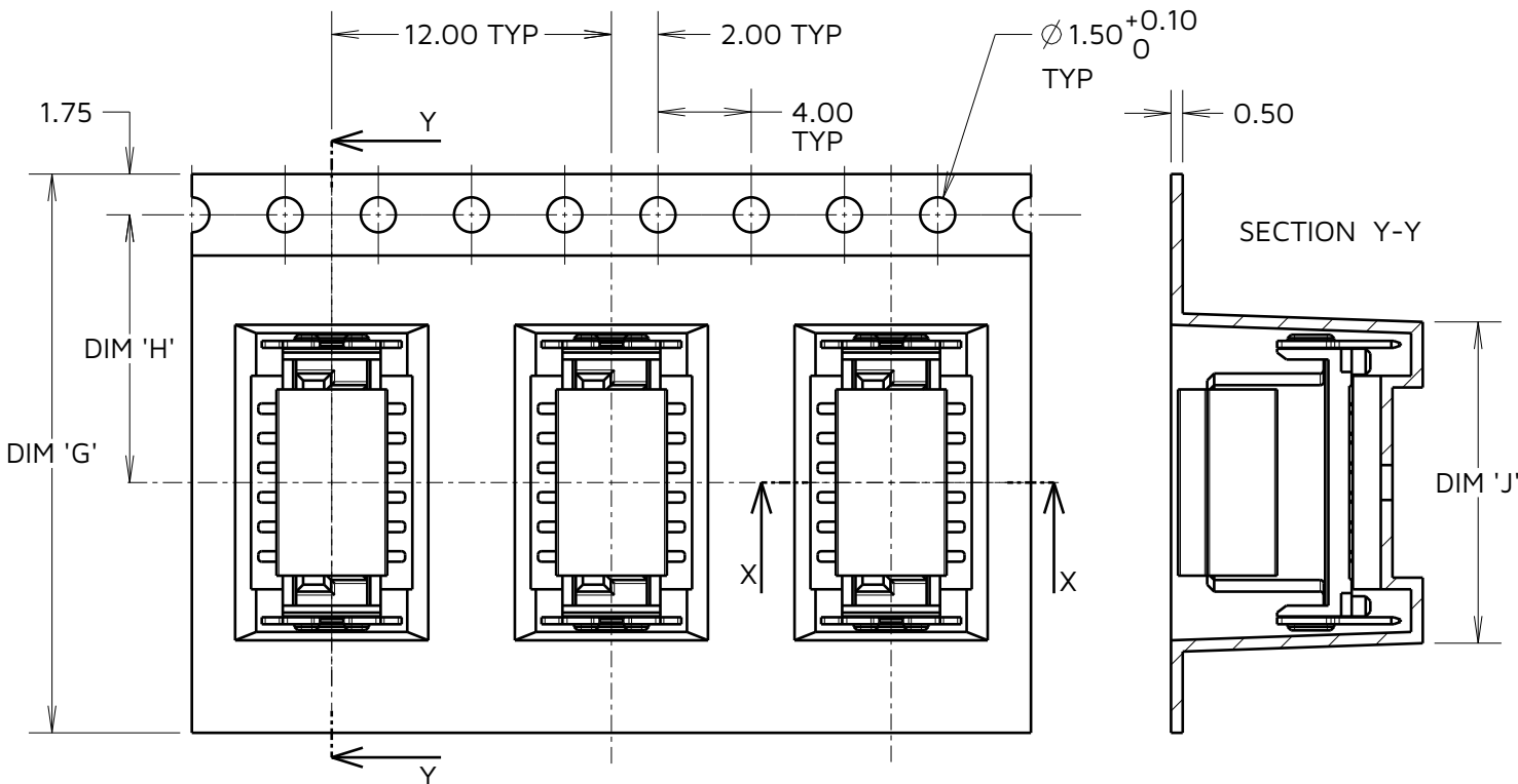
TAPE DETAILS FOR 12 TO 16 CONTACT CONNECTORS
