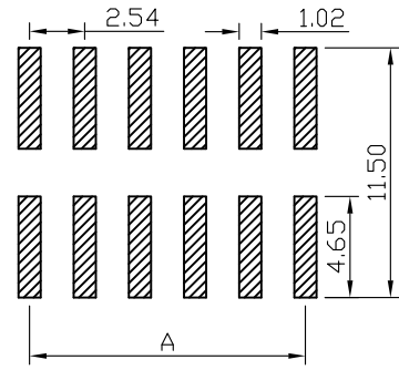
RECOMMEND P. C. B LAYOUT PCB TOLERANCE: ±0.05 (TOP VIEW)
