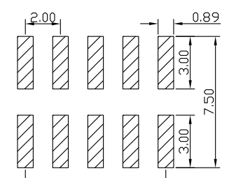
RECOMMEND P. C. B LAYOUT PCB TOLERANCE: ±0.05 (TOP VIEW)
