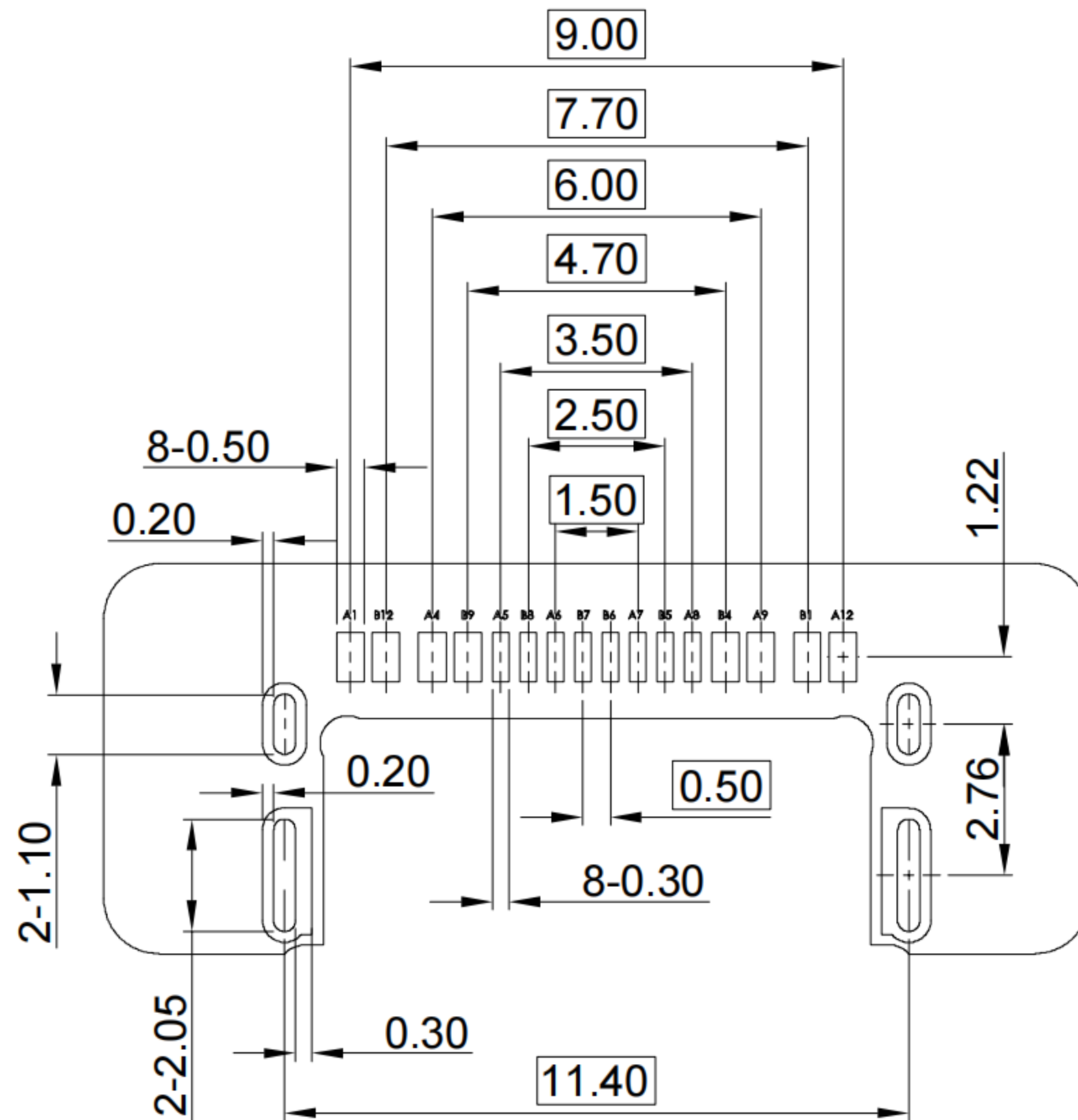
RECOMMENDED PCB LAYOUT TOLERANCE:±0.05
