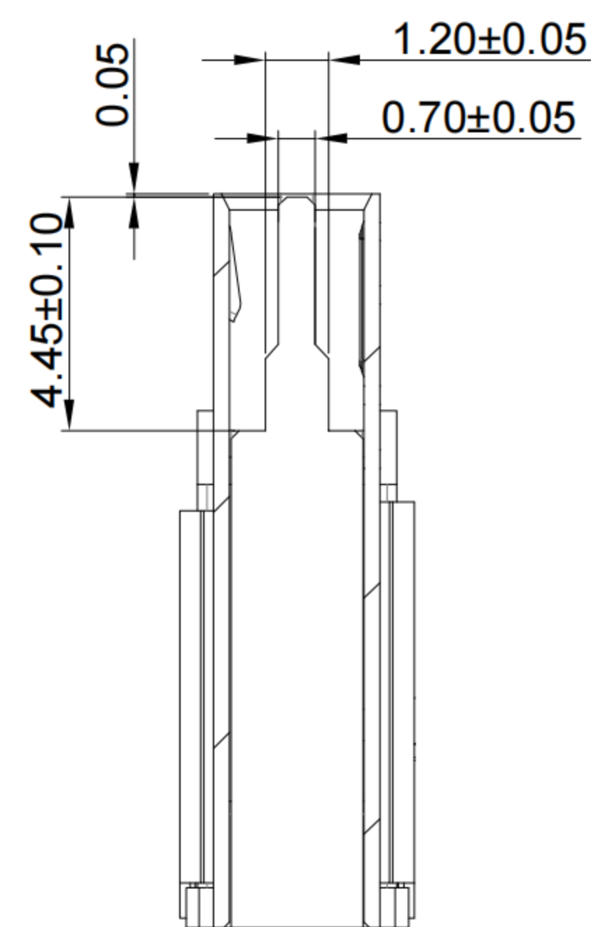
CUTAWAY VIEW
