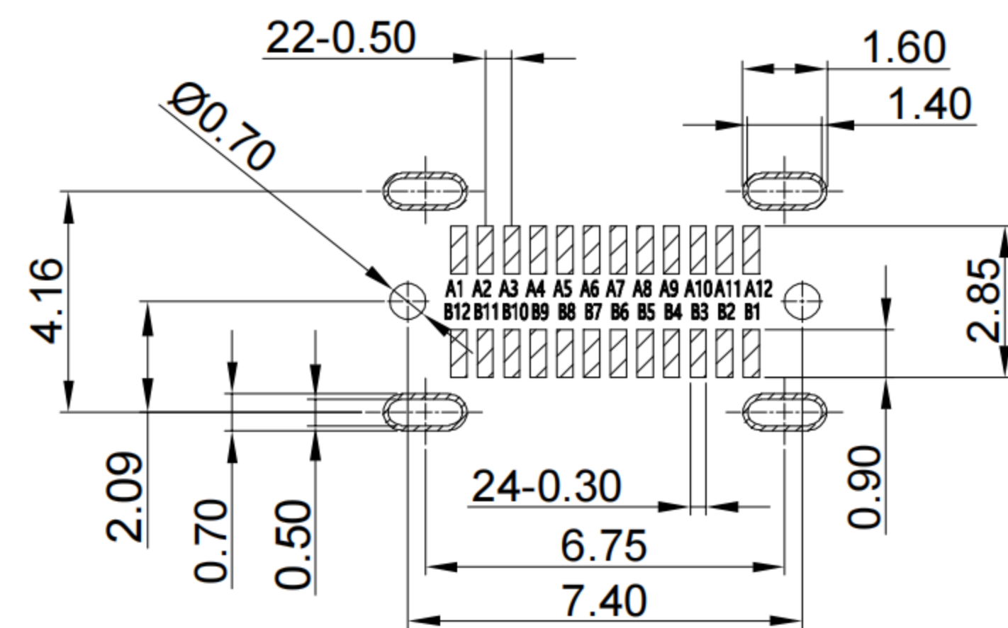
RECOMMENDED PCB LAYOUT TOLERANCE ±0.05mm
