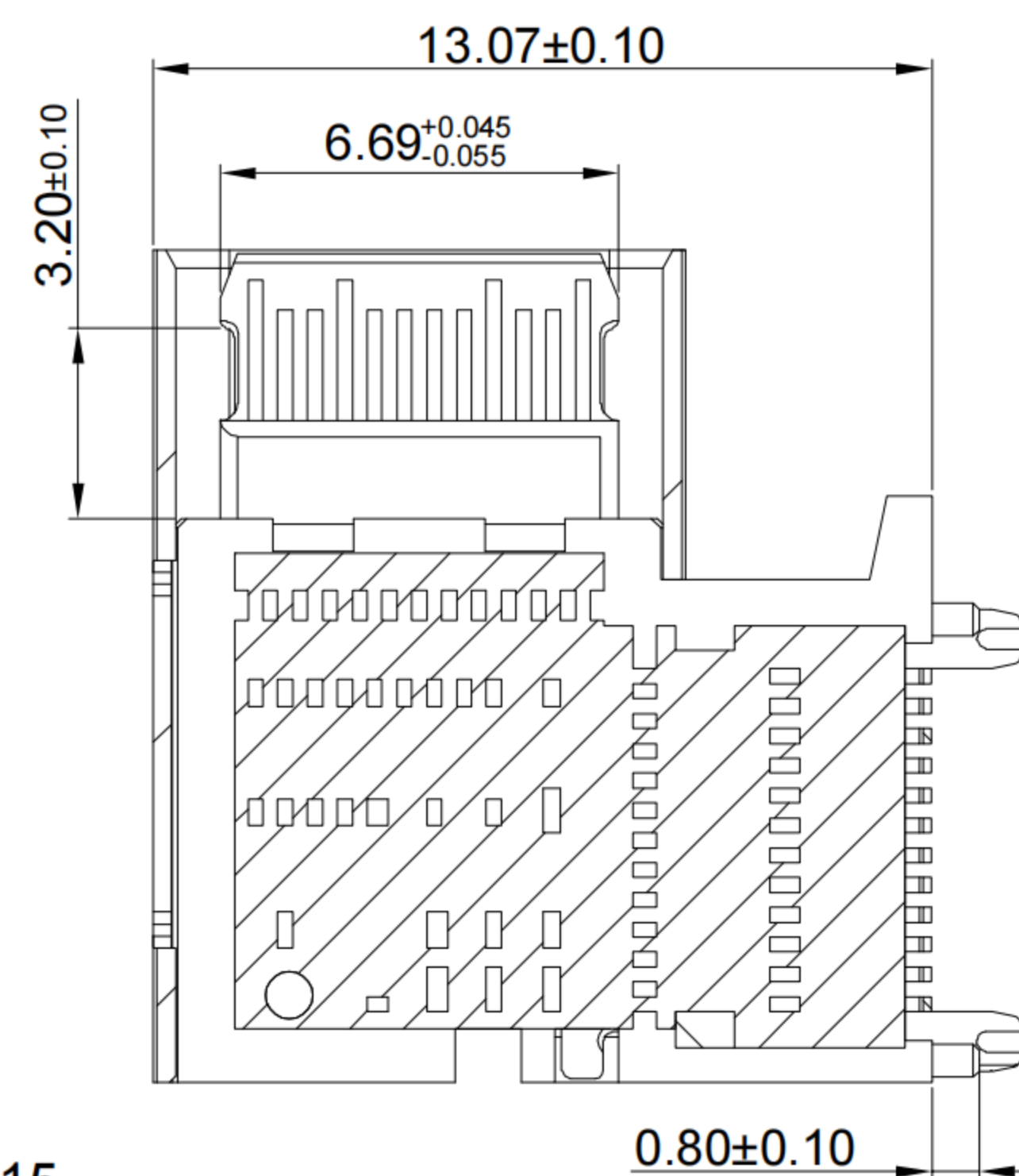
CUTAWAY VIEW
