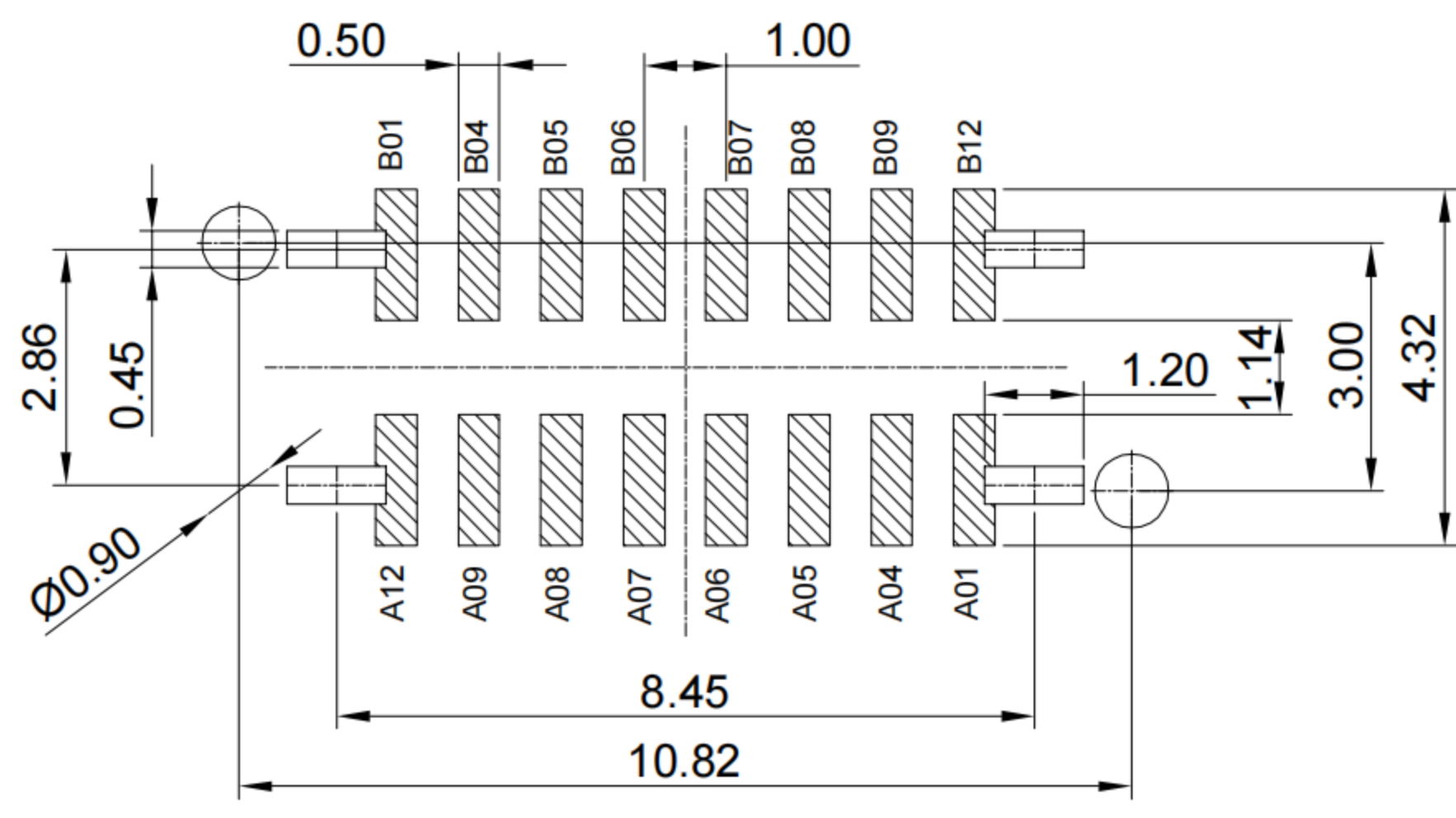
RECOMMENDED PCB LAYOUT TOLERANCE: ±0.05
