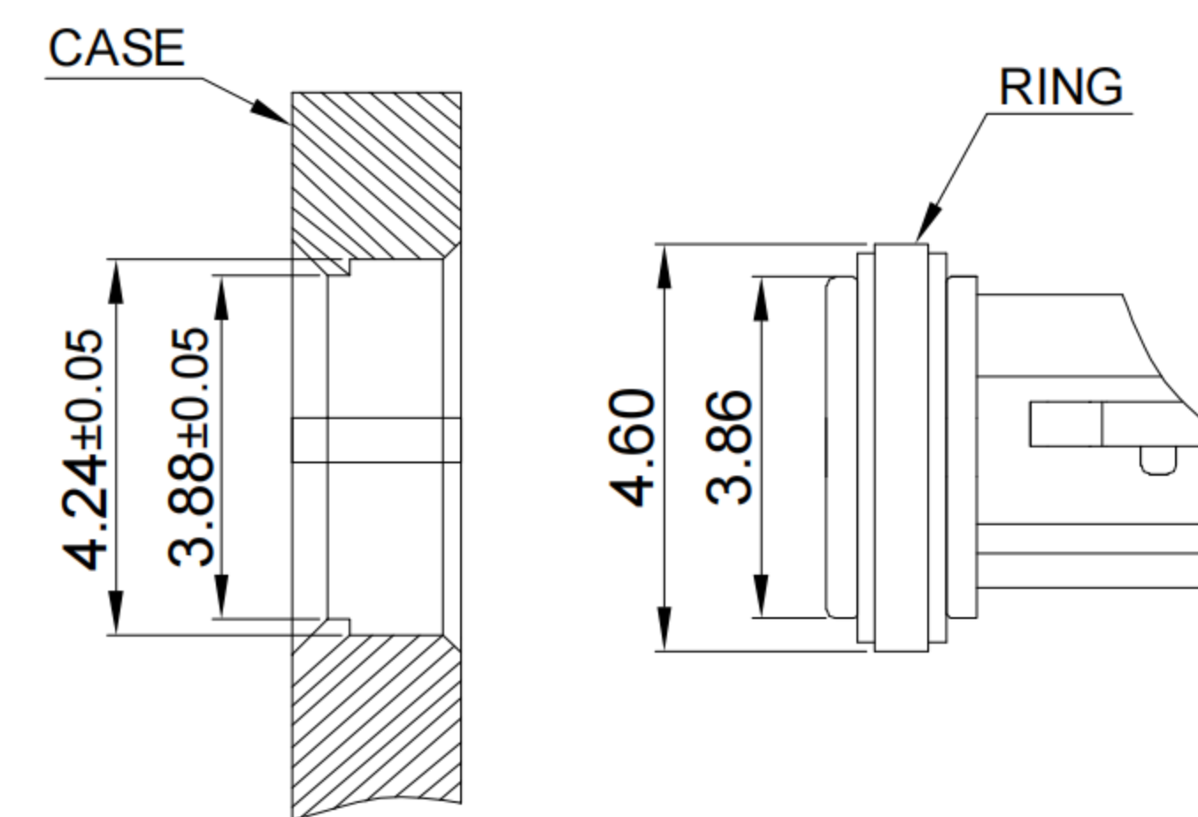
WATERPROOFING SCHEME FOR REFERENCE ONLY
