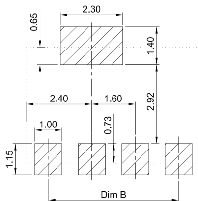
3&amp;4PIN LAYOUT
