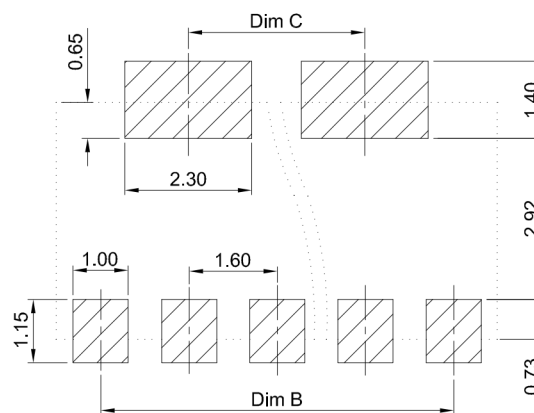
5-10PIN LAYOUT
