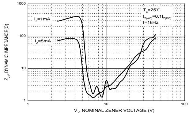
Effect of Zener Voltage on Zener Impedance
