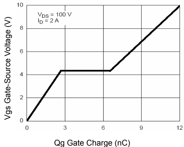
Figure 5 Gate Charge
