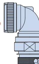
08 GR 90° Backshell with Rotating Coupling Nut Shrink Boot Adapter
