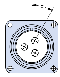
Alternate Position with Pin Contacts
