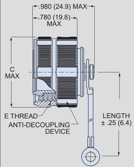
667-443 Receptacle Cover With Anti-Decoupling Device
