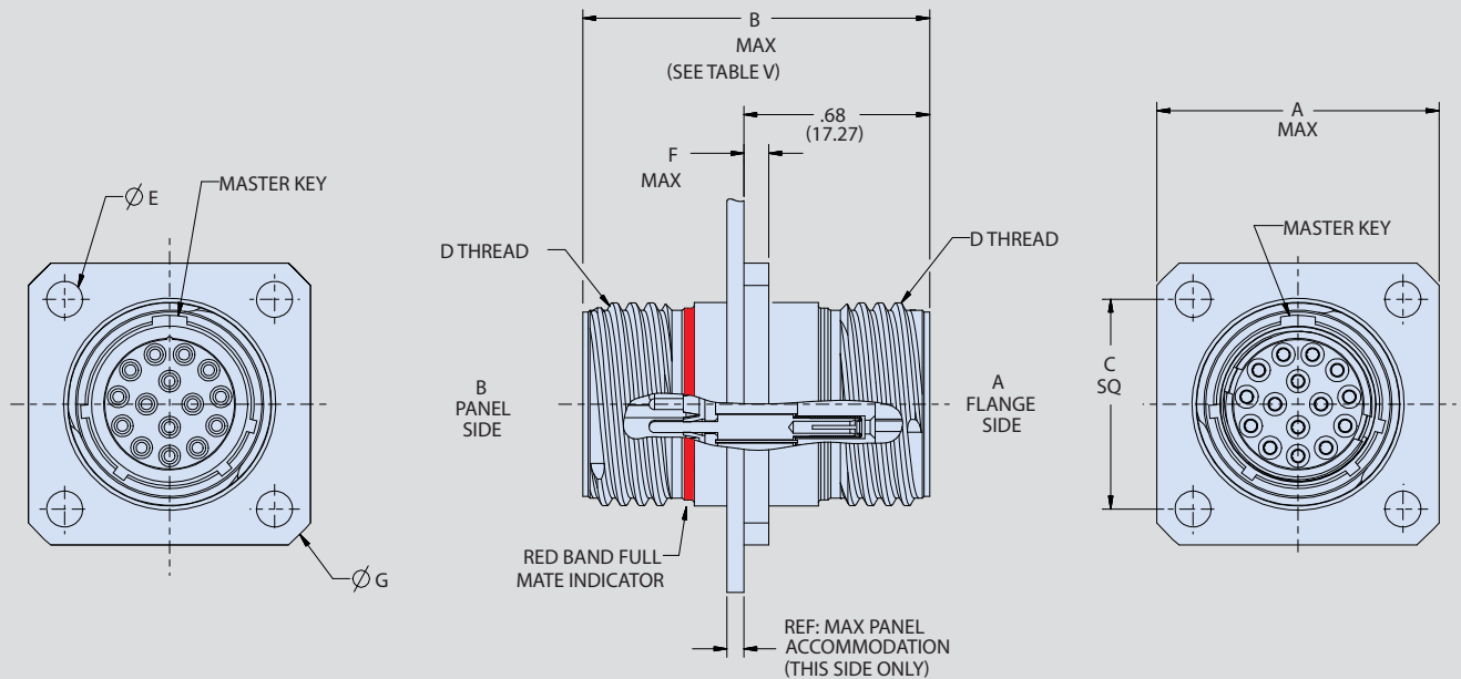
PANEL MOUNT INFO
