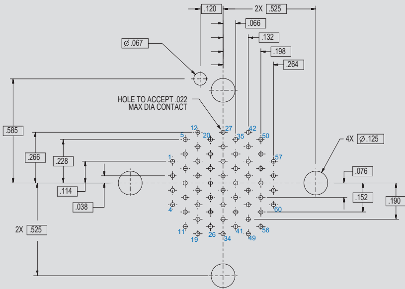
Arrangement No. 16-60 60x #22HD Contacts
