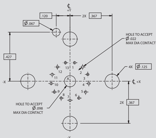
1x #12 and 13x #22HD Contacts
