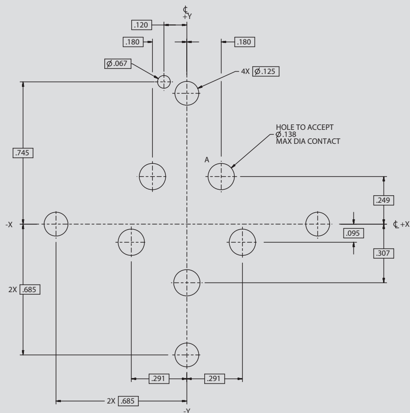
Arrangement No. 22-5 5x #8 Contacts
