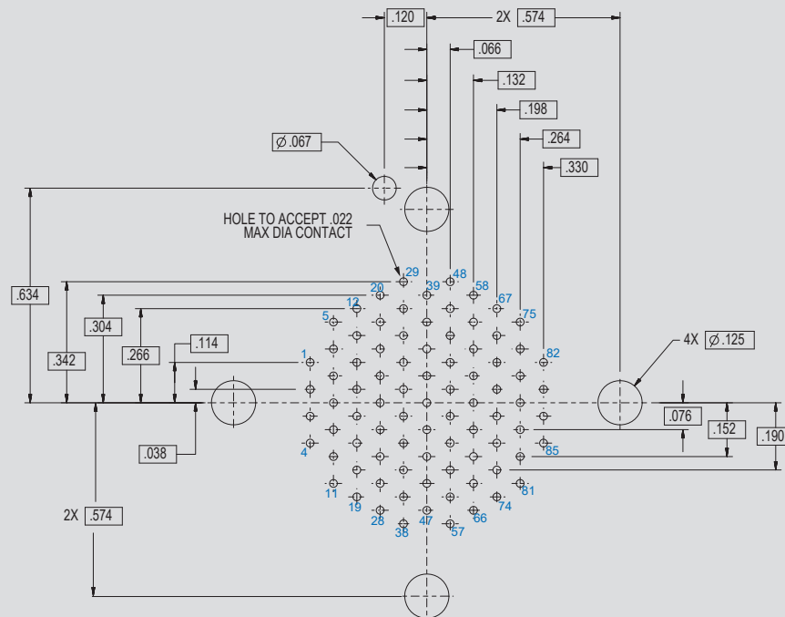
Arrangement No. 18-85 85x #22HD Contacts
