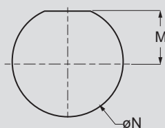
Jam-Nut Cutout
