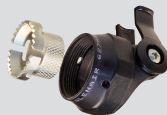
627V234 Low-Profile Swing-Arm® Flex with Drop-in EMI Adapter Page 130
