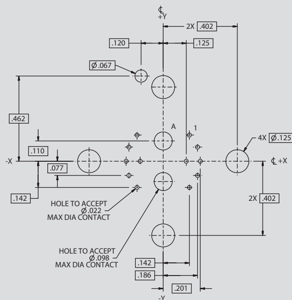
2x #12 and 12x #22HD Contacts
