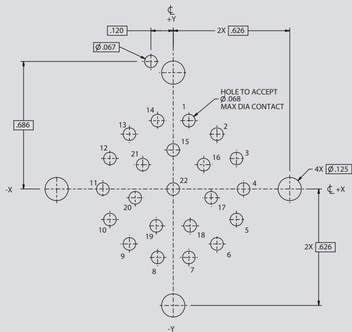
Arrangement No. 20-22 22x #16 Contacts
