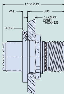
04- Jam Nut Receptacle with Wire Holes
