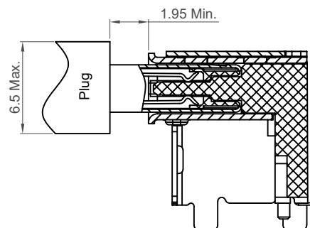
Plug and Receptacle Mating View
