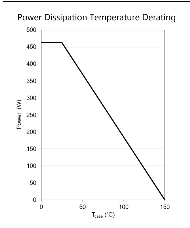
Figure 14: Power Derating vs. T_{case}
