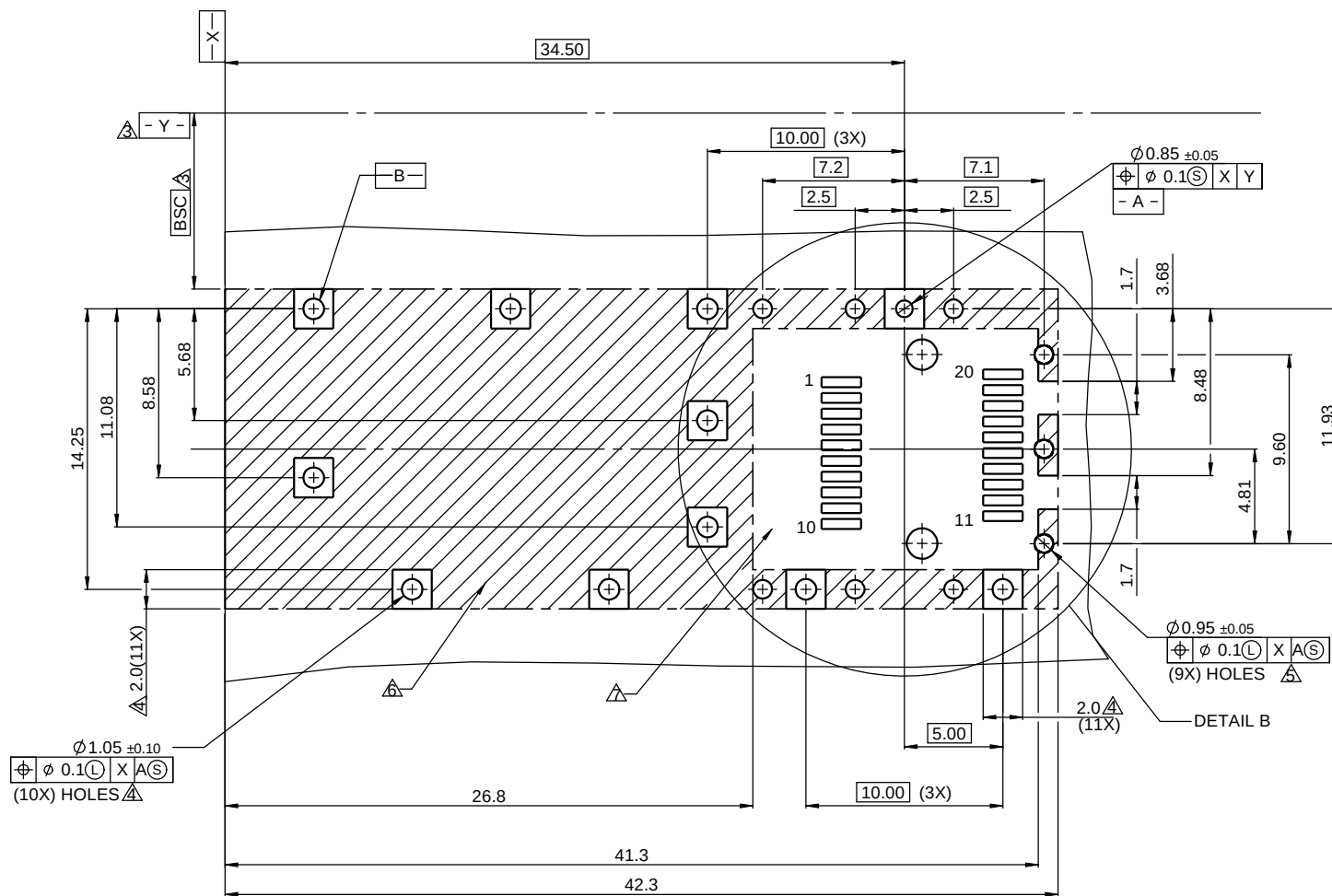
SFP HOST BOARD MECHANICAL LAYOUT
