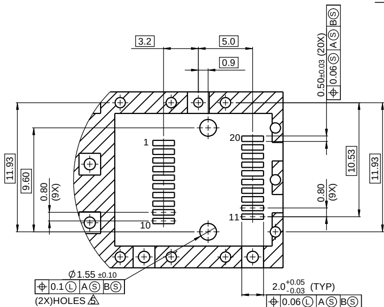
DETAIL B
