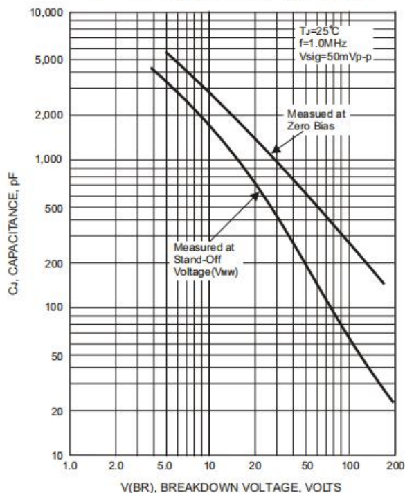
FIG.4-TYPICAL JUNCTION CAPACITANCE
