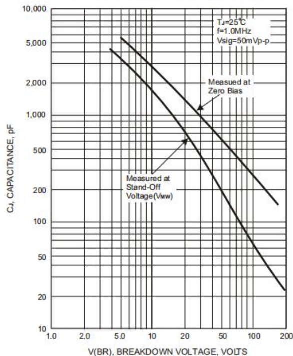
FIG.4-TYPICAL JUNCTION CAPACITANCE
