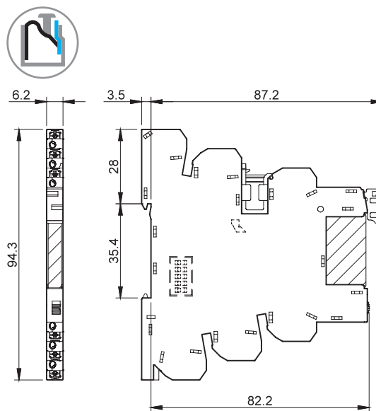
Types 39.90 39.91 Push-in terminal
