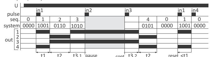
time [4 sequence]
