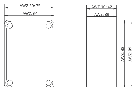
surface-mounted for: AWZ, AWZ-30
