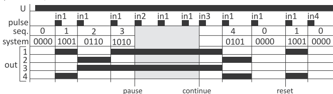
pulse [4 sequence]
