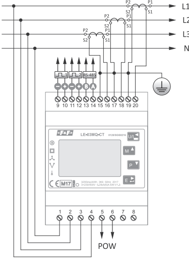
3×230 V+N 3-phase 4-wire installation
