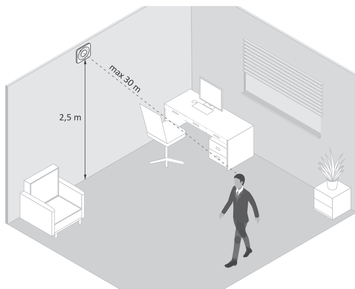
Detection field range (wall mounting)
