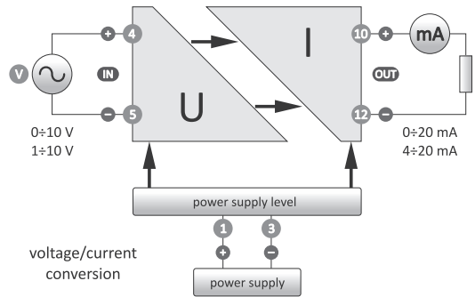
Voltage/current
