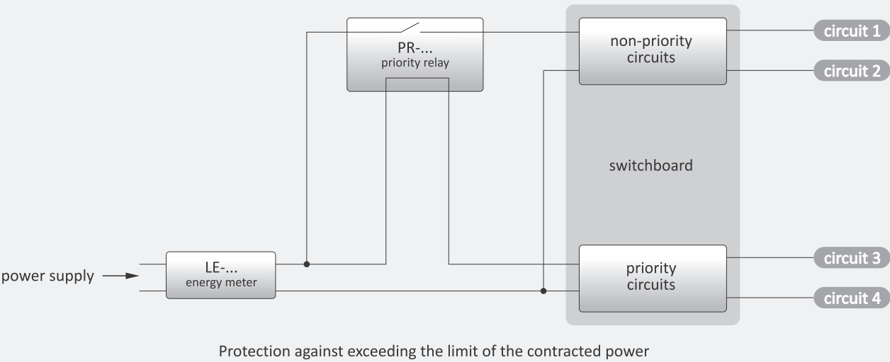
Protection against exceeding the limit of the contracted power
