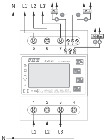
3×400 V 3-phase 3-wire installation (without neutral wire)
