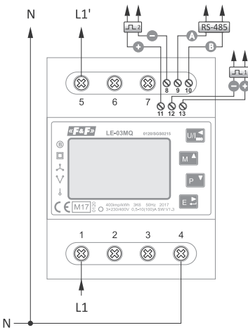
230 V AC 1-phase 2-wire installation
