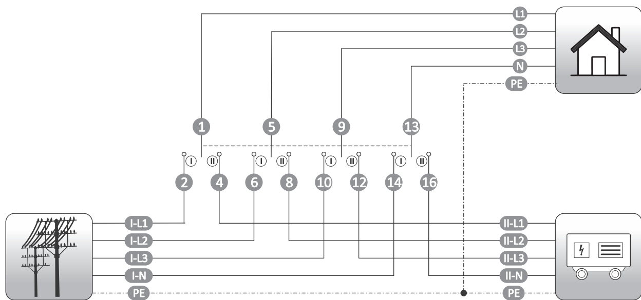
Wiring diagram
