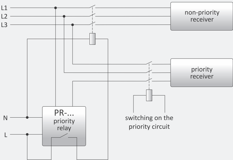
Use of the PR in the symmetrical three-phase receiver system
