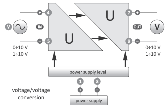
Voltage/voltage
