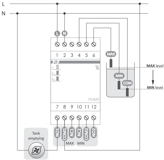
Tank emptying
