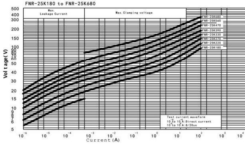
V-I Curve
