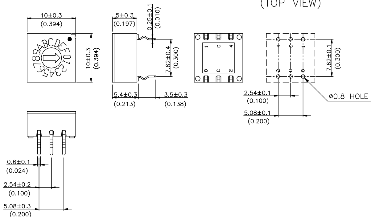
P.C.B. LAYOUT (TOP VIEW)
