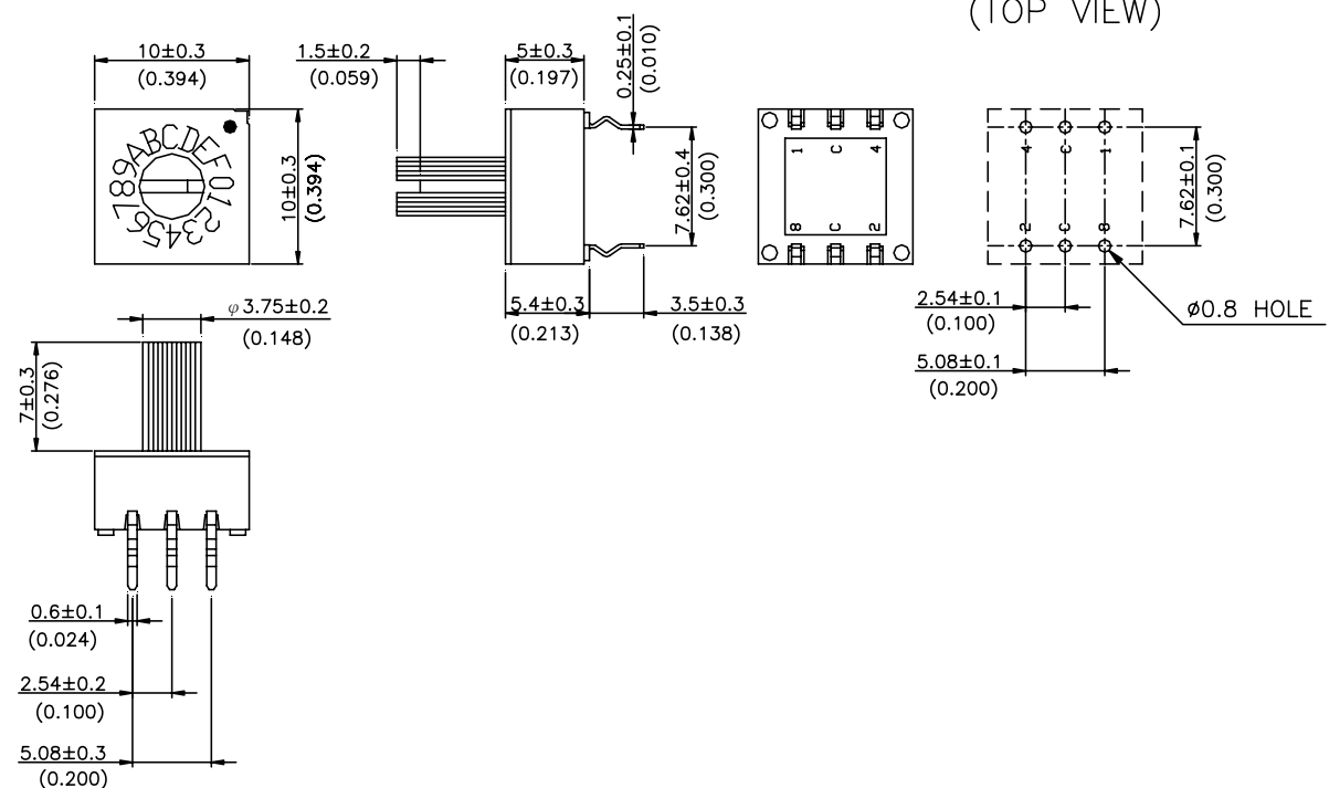
ERD2XXS Shaft Type
