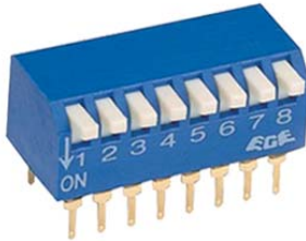
EPG/EPS SPST
