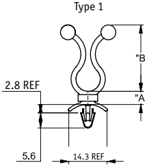
Type 1 Bottom Hole: Snap-lock Ø 4 ± 0.08 Panel Thickness: 0.8-2
