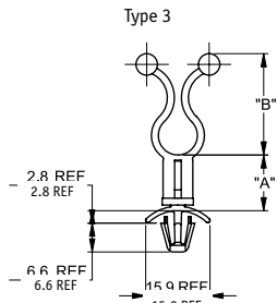
Type 3 Bottom Hole: Snap-lock Ø 6 ± 0.08 Panel Thickness: 0.8-2
