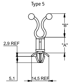
Bottom Hole: Snap-lock 5.5 square Panel Thickness: 0.8-2
