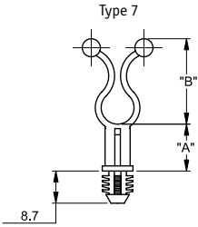
Bottom Hole: Press-fit Ø 8.0 ± 0.08 Panel Thickness: 6.4 Min.
