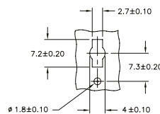
MOUNTING HOLE DETAIL
