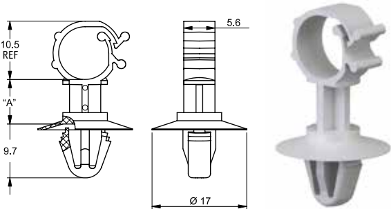
Bottom Hole: Snap-lock 6.5-7 Panel Thickness: 0.8-1.25
