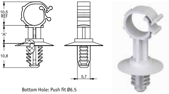
Bottom Hole: Push fit Ø6.5 Panel Thickness: Min 0.7
