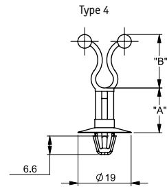
Type 4 Bottom Hole: Snap-lock Ø 6.5 ± 0.09 Panel Thickness: 0.8-1.6
