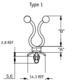
Type 1 Bottom Hole: Snap-lock Ø 4 ± 0.08 Panel Thickness: 0.8-2
