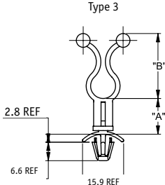
Type 3 Bottom Hole: Snap-lock Ø 6 ± 0.08 Panel Thickness: 0.8-2
