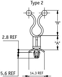
Type 2 Bottom Hole: Snap-lock Ø 4.75 ± 0.08 Panel Thickness: 0.8-2
