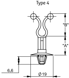
Type 4 Bottom Hole: Snap-lock Ø 6.5 ± 0.09 Panel Thickness: 0.8-1.6
