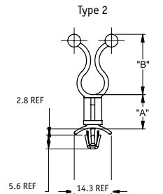
Type 2 Bottom Hole: Snap-lock Ø 4.75 ± 0.08 Panel Thickness: 0.8-2
