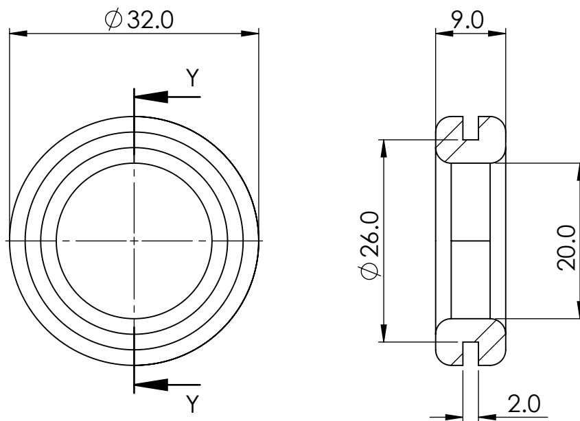
SECTION Y-Y
