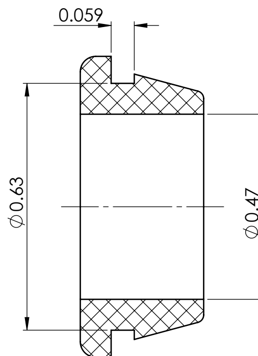
SECTION Y-Y
