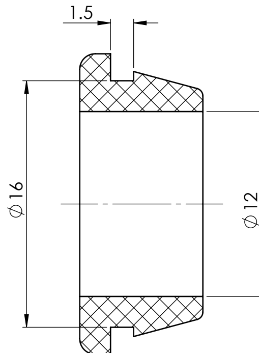
SECTION Y-Y
