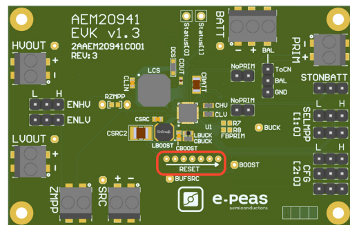
Figure 2: Board reset
