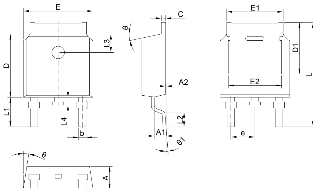
COMMON DIMENSIONS CUNITS MEASURE=MILLIMETER
