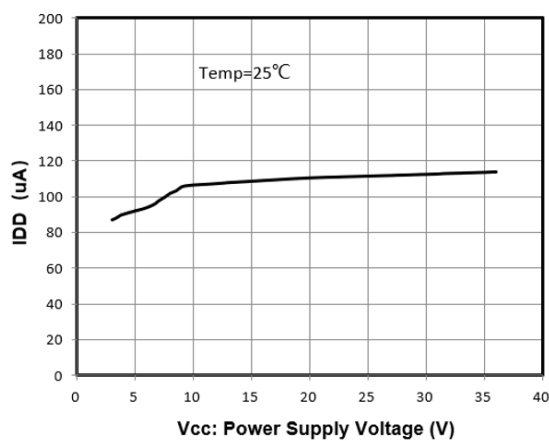
Figure 6. Quiescent Current vs. Power Supply Voltage
