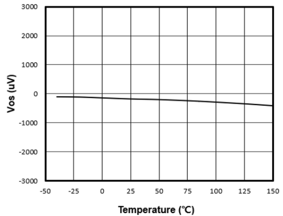
Figure 4. Offset Voltage vs. Temperature
