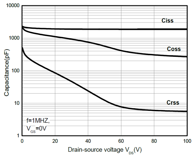
Figure 7. Capacitance Characteristics
