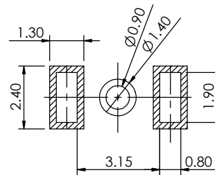
PCB LAYOUT TOLERANCE: ±0.05
