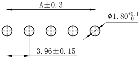
PCB LAYOUT
