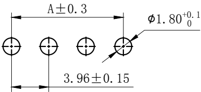
PCB LAYOUT
