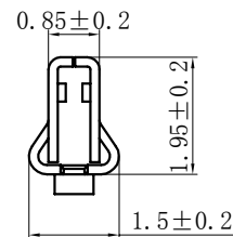
SECTION C-C
