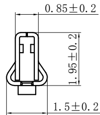
SECTION C
