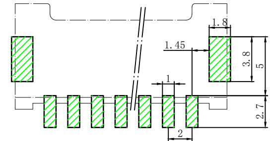
PCB LAYOUT
