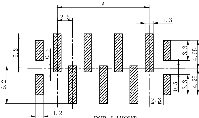
PCB LAYOUT
