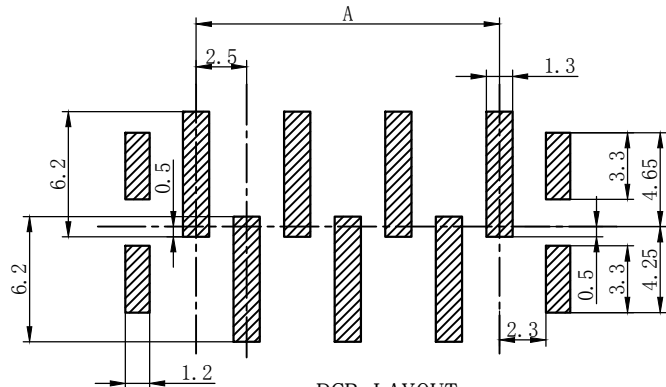
PCB LAYOUT
