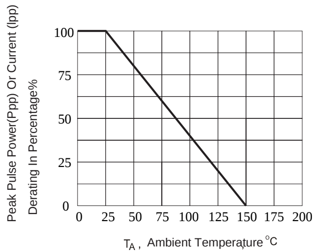
Fig.1 Derating Curve
