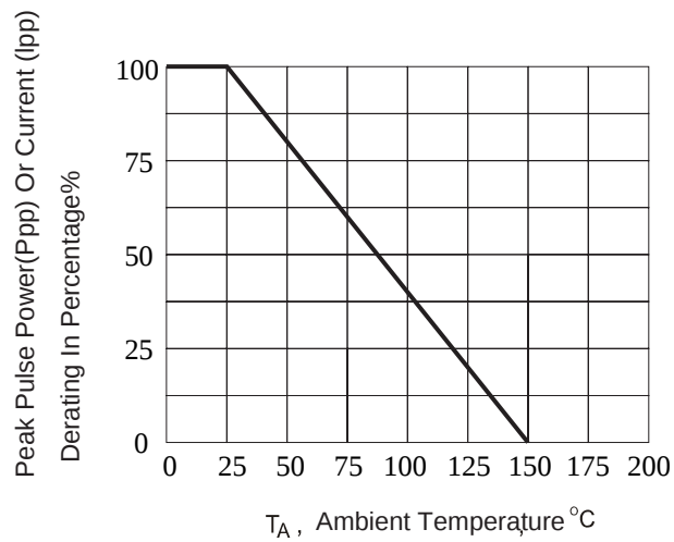
Fig.1 Derating Curve
