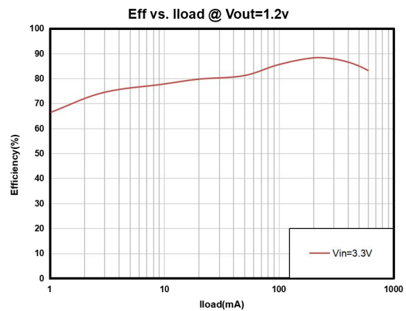
Figure 6. Efficiency vs. I_{load} at V_{OUT} = 1.2\text{ V}
