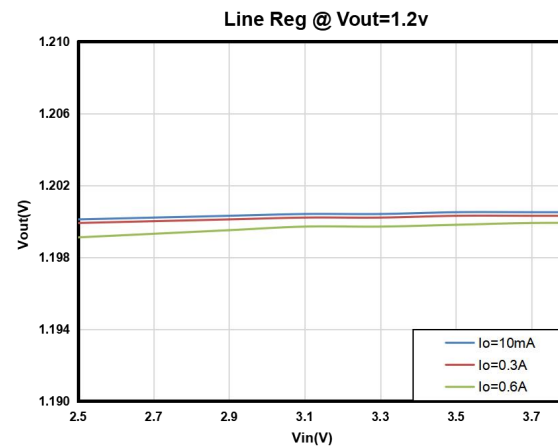
Figure 14. Output voltage vs. Input voltage
