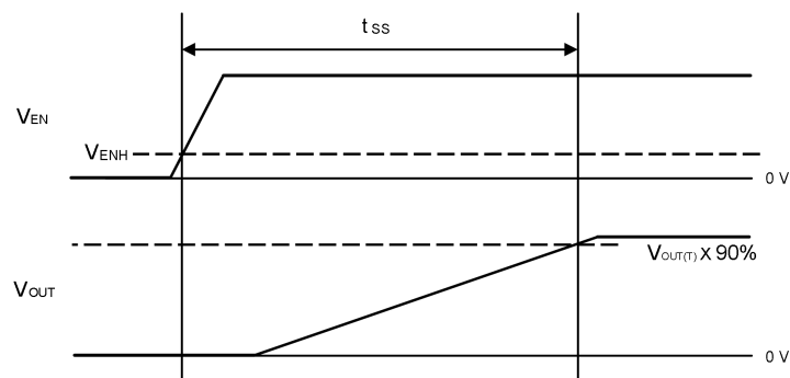
Figure 35. Soft-start
