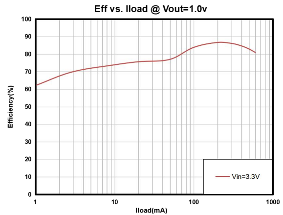
Figure 4. Efficiency vs. I_{load} at V_{OUT} = 1.0\text{ V}
