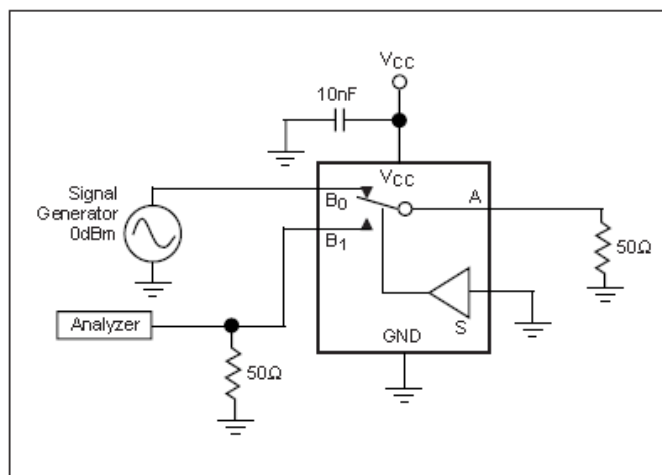
Figure 6. Crosstalk
