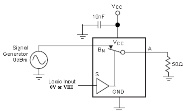
Figure 9. Bandwidth
