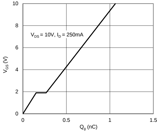
Figure 21. Gate Charge (Q1)
